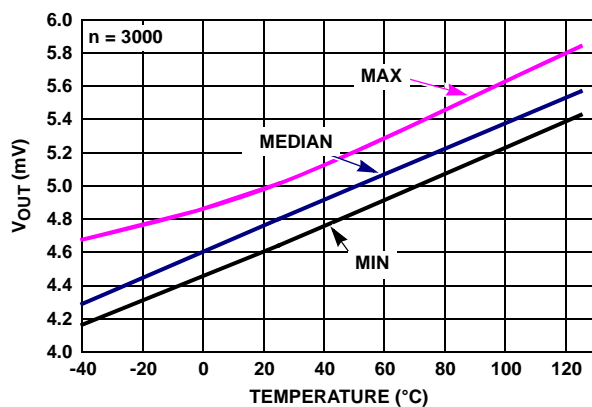
FIGURE 35. ISL28271 V_{OUT} LOW vs TEMPERATURE, R_L = 100k , V_+ = \pm 2.5V
