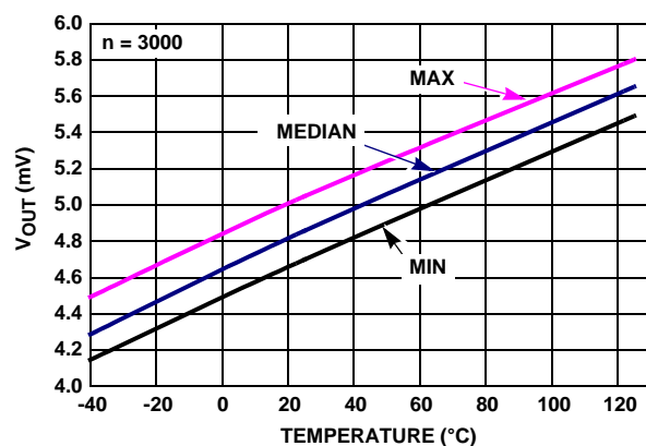
FIGURE 36. ISL28272 V_{OUT} LOW vs TEMPERATURE, R_L = 100k , V_+ = \pm 2.5V
