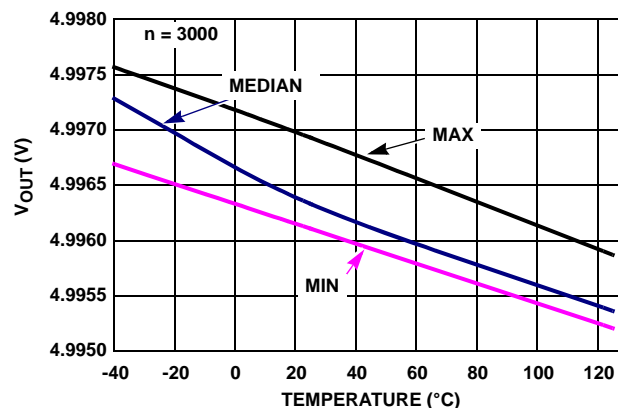
FIGURE 32. ISL28272 V_{OUT} HIGH vs TEMPERATURE, R_L = 100k , V_+ = \pm 2.5V
