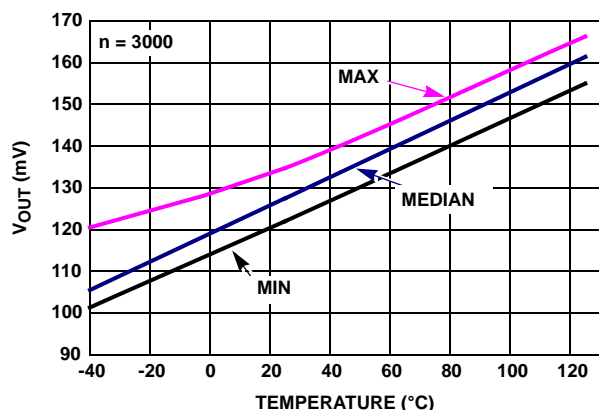
FIGURE 33. ISL28271 V_{OUT} LOW vs TEMPERATURE, R_L = 1k , V_+ = \pm 2.5V
