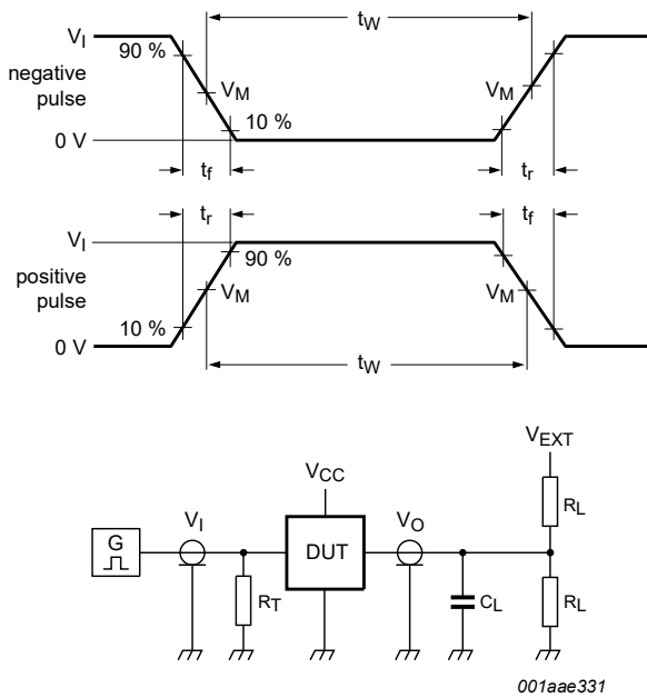
Test data is given in Table 9 . Definitions test circuit: R_L = Load resistance; C_L = Load capacitance including jig and probe capacitance; R_T = Termination resistance should be equal to output impedance Z_o of the pulse generator; V_{EXT} = Test voltage for switching times.
