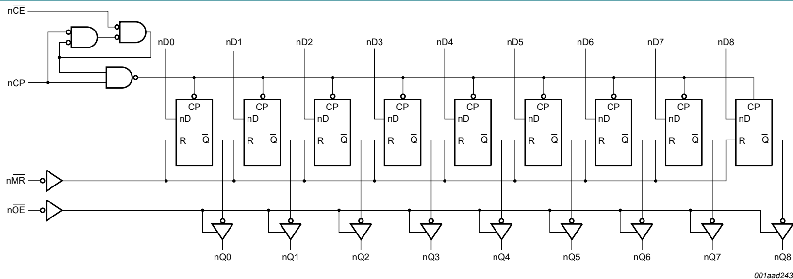
Fig. 3. Logic diagram
