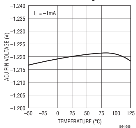
LT1964 ADJ Pin Voltage
