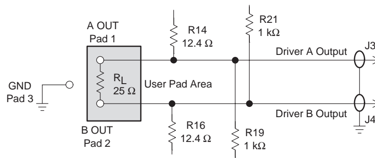
Figure 1–7. THS6002 EVM Driver Frequency Response Test Circuit
