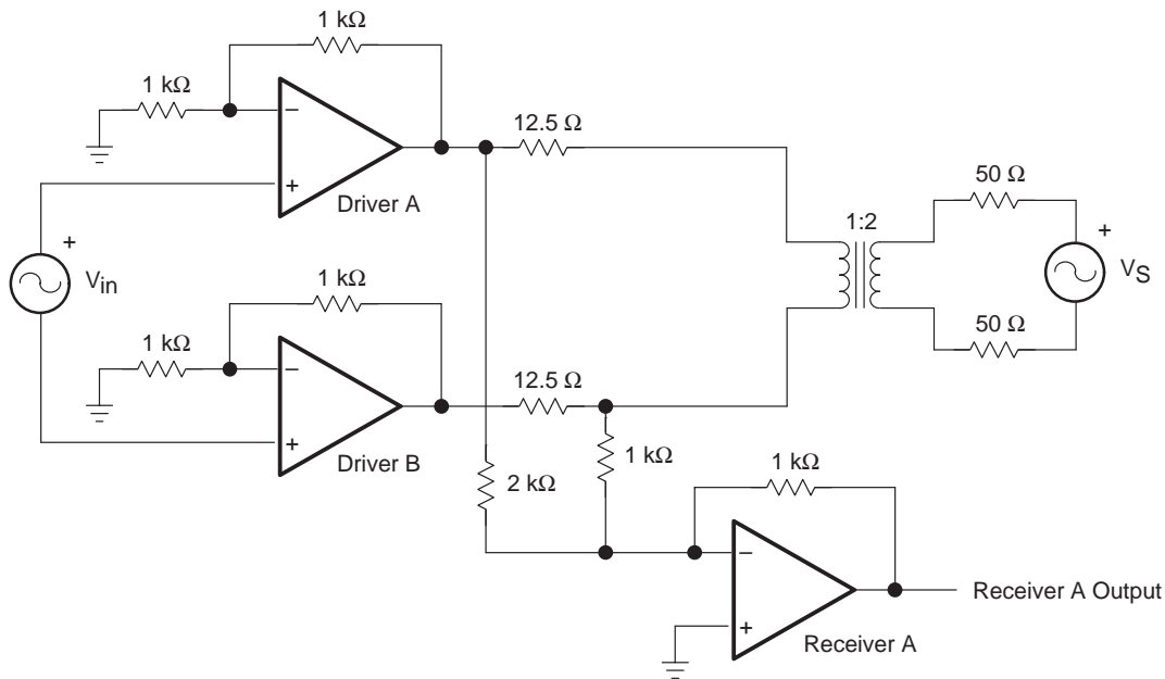
Figure 1–4. Receiver Analysis Schematic
