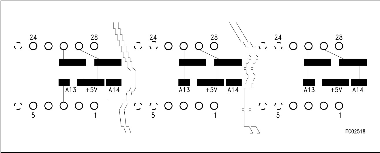
Figure 3 Solder straps underneath the EPROM to set the EPROM: Left 8 K EPROM (2764), middle 16 K EPROM (27128), right 32 K EPROM (27256) With version 3.1 of the SICOFI you may connect analog and digital ground with a solder strap between pins 3 and 5 of the SICOFI. The solder straps for the resistor in the SIP-line are close to the SICOFI (see figure 4).
