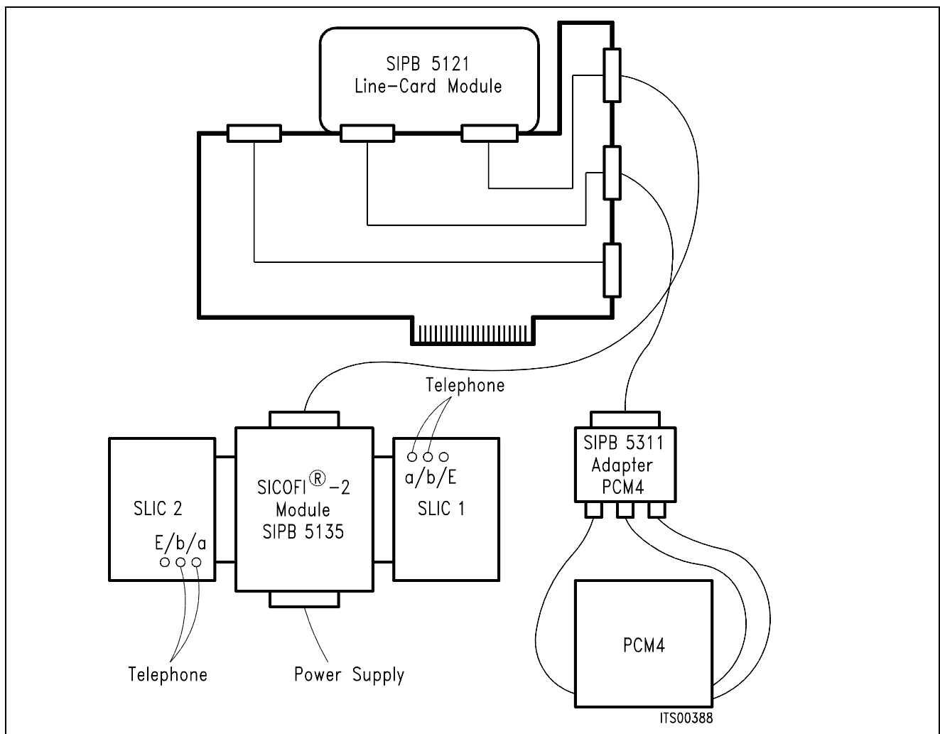
Figure 1 Measuring Set-Up
