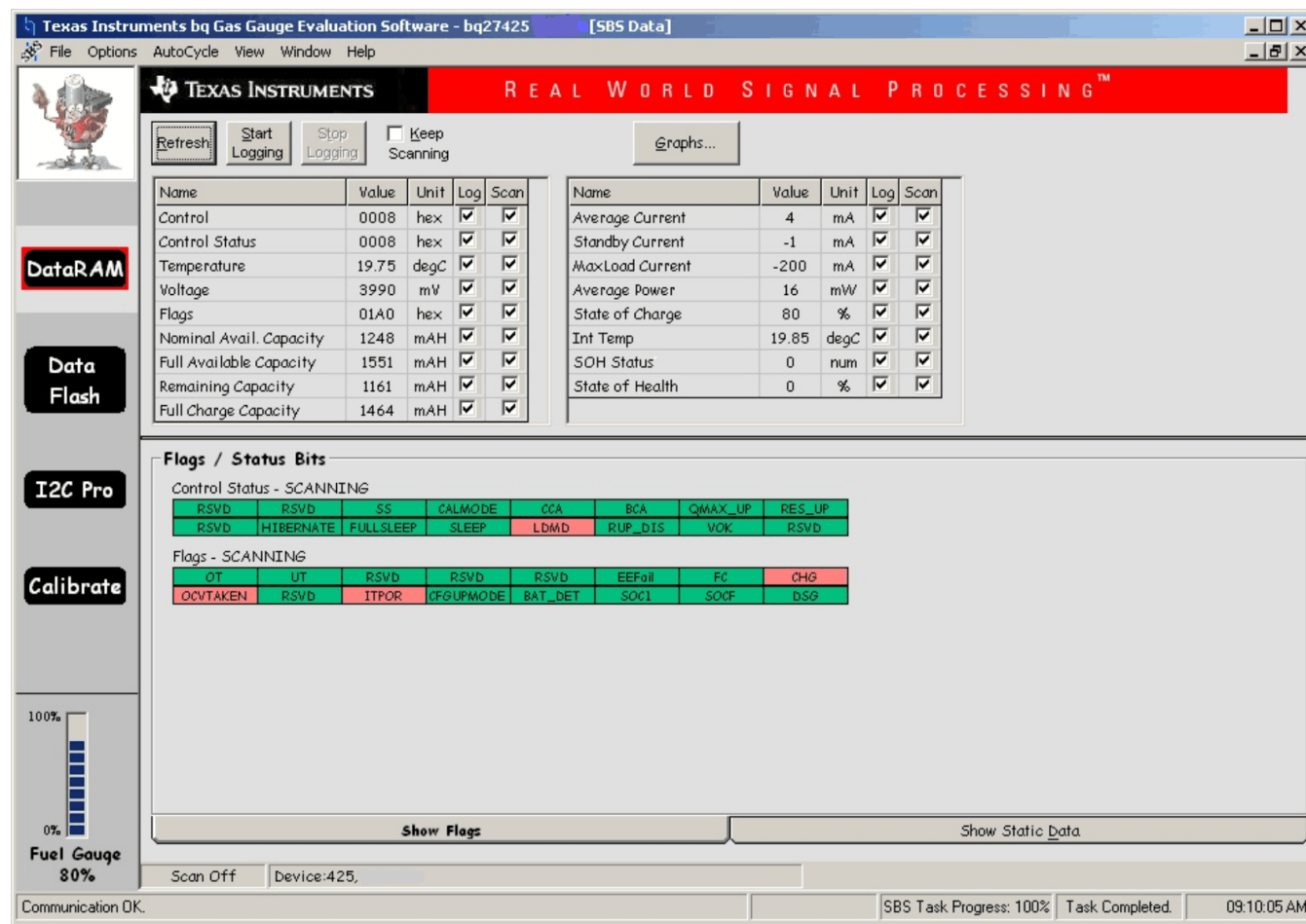
Figure 7. DataRAM Screen
