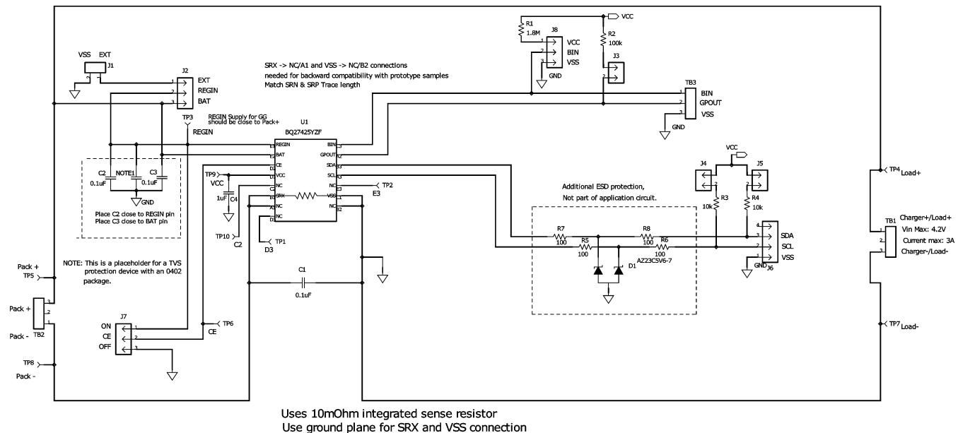
Figure 5. bq27425EVM Schematic
