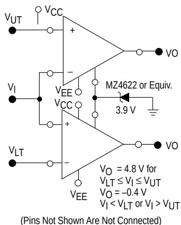
Figure 2. Double-Ended Limit Detector
