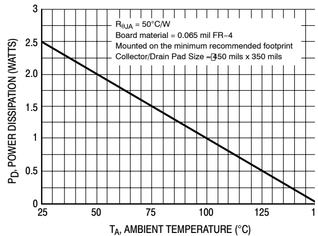
Figure 15. D²PAK Power Derating Curve
