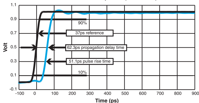
RF300 Time Response (RF Note 6)
