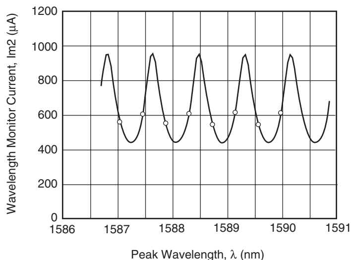
Fig. 5 Filter Curve
