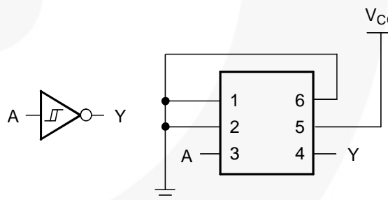
Figure 7. Inverter
