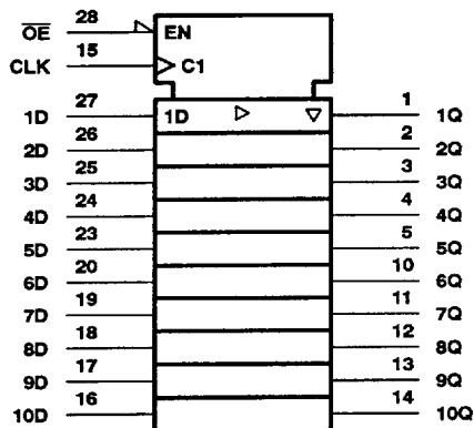
logic symbol†
