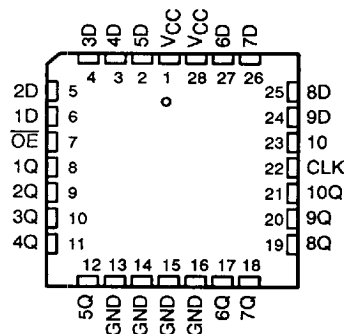
54ACT11821 ... FK PACKAGE (TOP VIEW)
