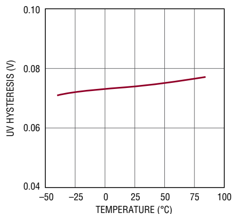
\overline{\text{EN1}} , \overline{\text{EN2}} Hysteresis vs Temperature
