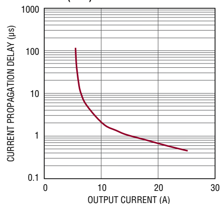
Current Limit Delay ( t_{PHL(ILIM)} ) vs Overdrive
