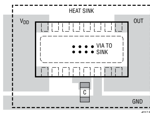
Figure 6. Recommended Layout
