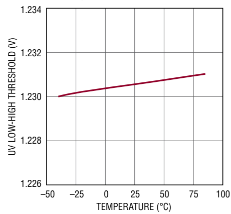
\overline{\text{EN1}} , \overline{\text{EN2}} Low Threshold vs Temperature
