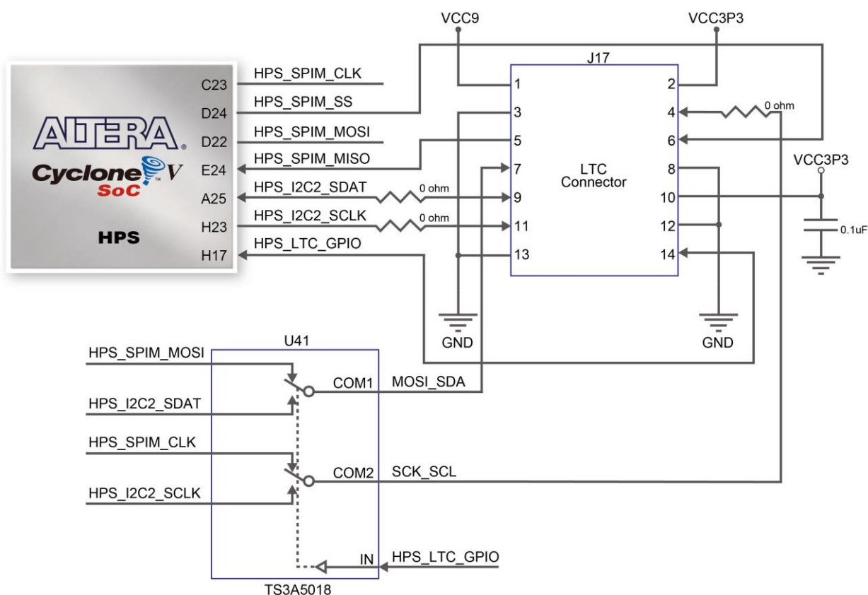
Figure 3-36 Connections between the HPS and LTC connector
