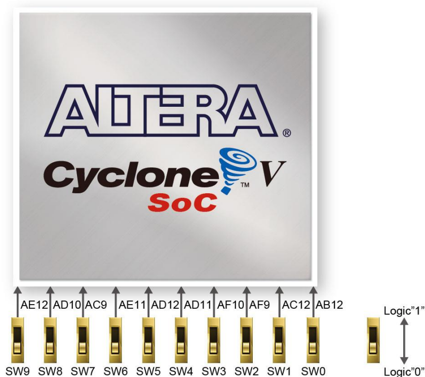
Figure 3-15 Connections between the slide switches and the Cyclone V SoC FPGA
