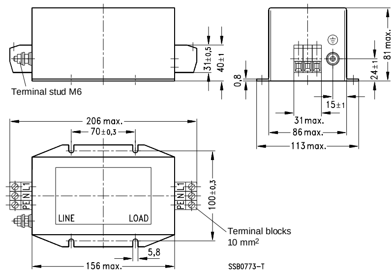
Outline drawing B84142-B25-R
