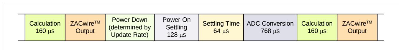
Figure 3.9 ZACwire TM Output Timing for Lower Update Rates
