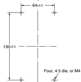
Mounting Holes
