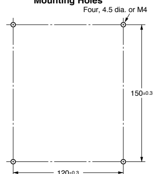
Mounting Holes
