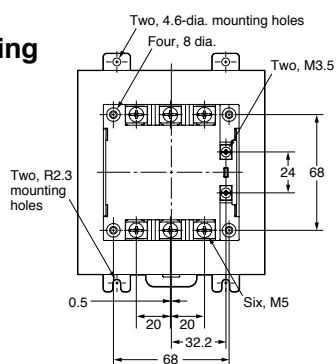
Mounting Holes
