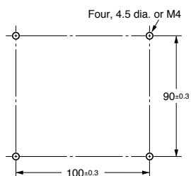
Mounting Holes
