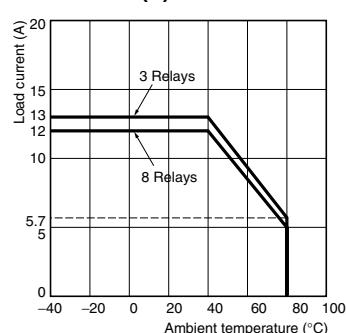
G3PE-515B(L)
