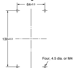
Mounting Holes
