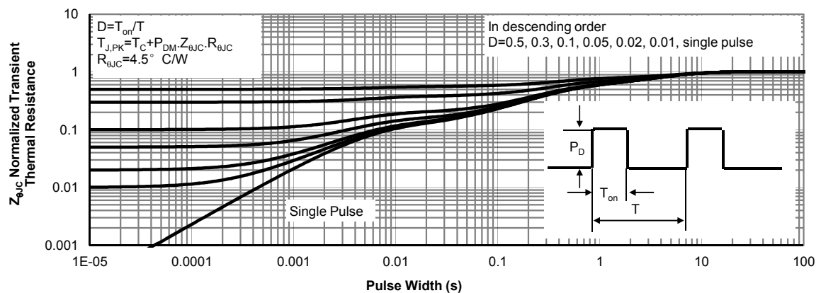
Figure 11: Normalized Maximum Transient Thermal Impedance for AOWF9N70 (Note F)
