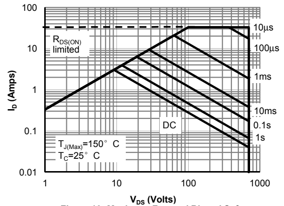
Figure 10: Maximum Forward Biased Safe Operating Area for AOWF9N70 (Note F)
