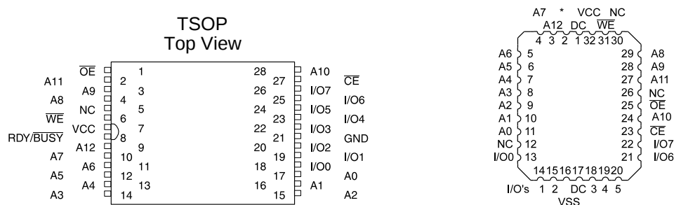
LCC, PLCC Top View
