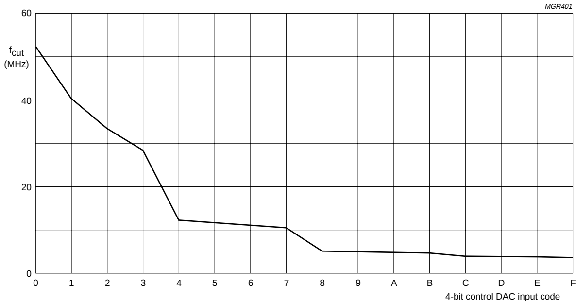
Fig.13 AGC bandwidth.
