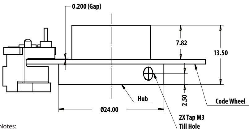
Figure 3. Encoder module with codewheel dimensions
