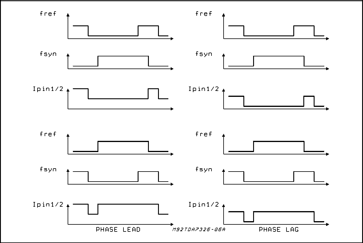
Figure 4: Phase comparator
