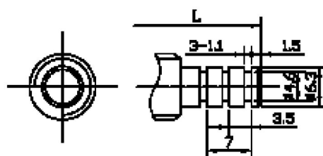
METAL SHAFT (T TYPE)
