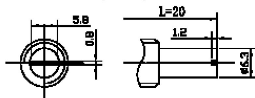
PLASTIC SHAFT (M TYPE)
