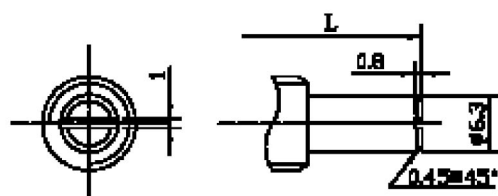
METAL SHAFT (U TYPE)
