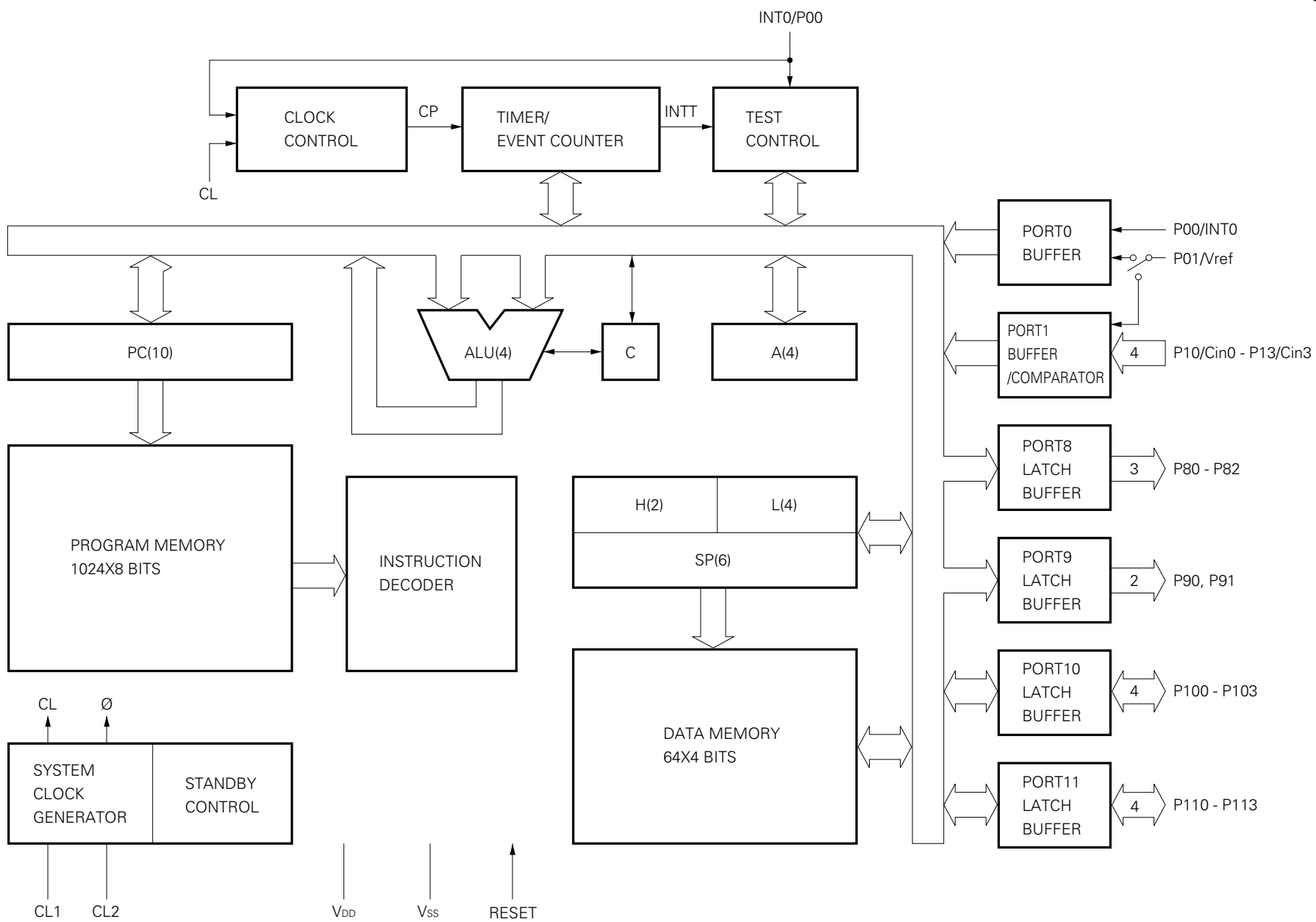
μPD7566A BLOCK DIAGRAM
