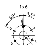
Drilling diagram for 60° indexing angle
