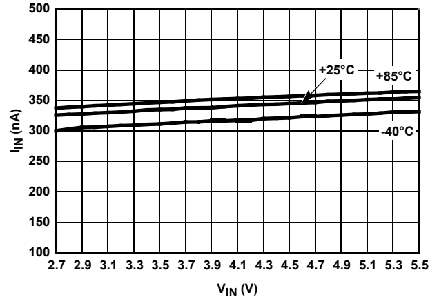
FIGURE 43. I_{IN} vs V_{IN} OVER-TEMPERATURE
