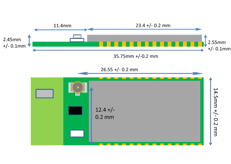
Figure 11: Dimensions of WT11u-E
