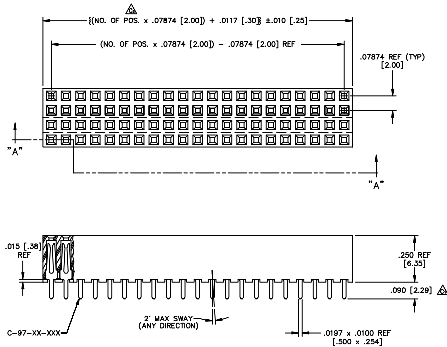
SECT. "A-A"
