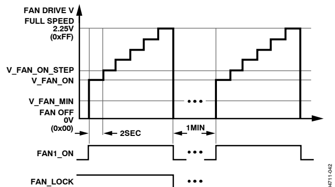
Figure 43. Abnormal Fan Starting (Fan Stalled)
