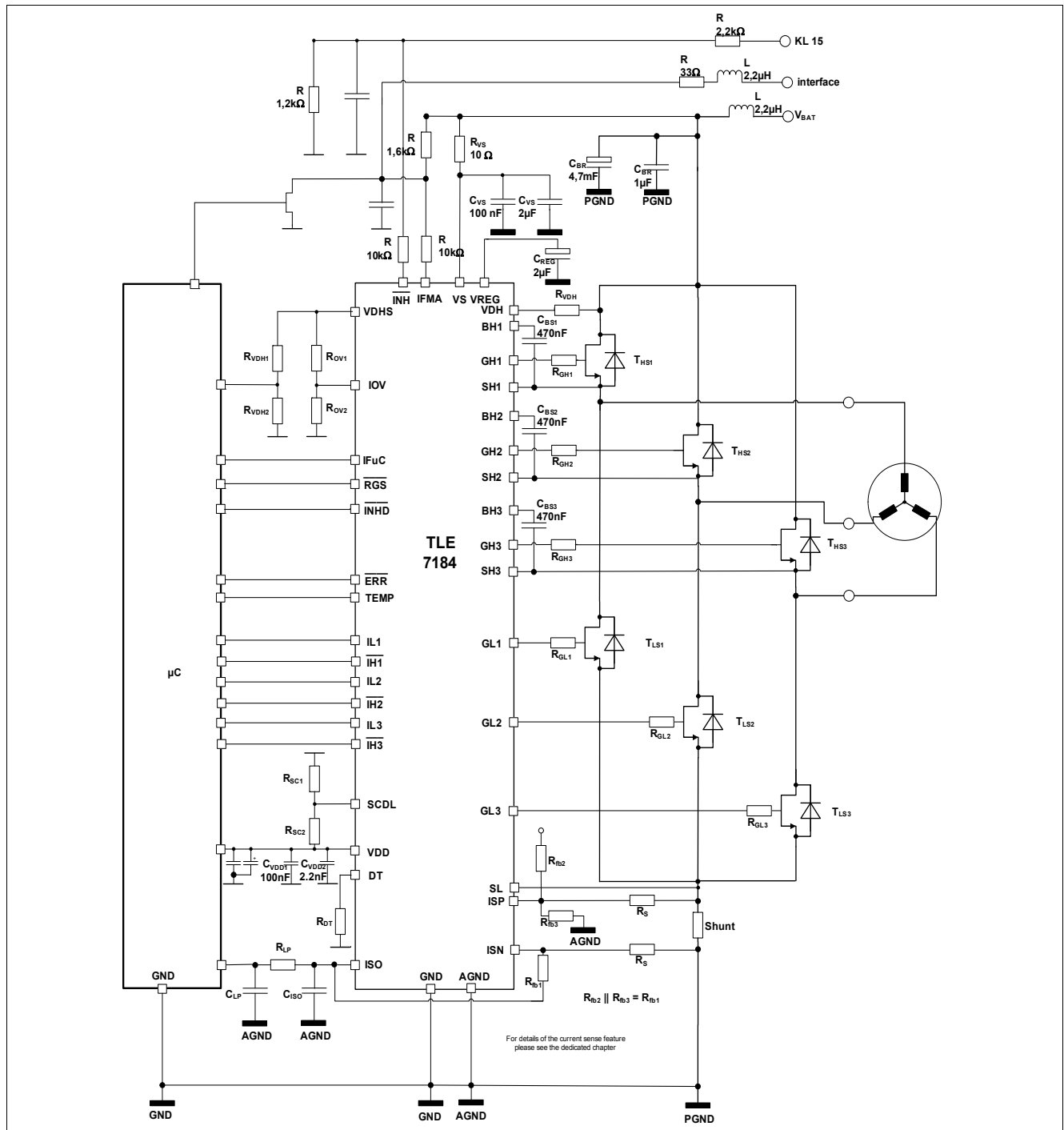
Figure 14 Application Circuit TLE7184F-3V
