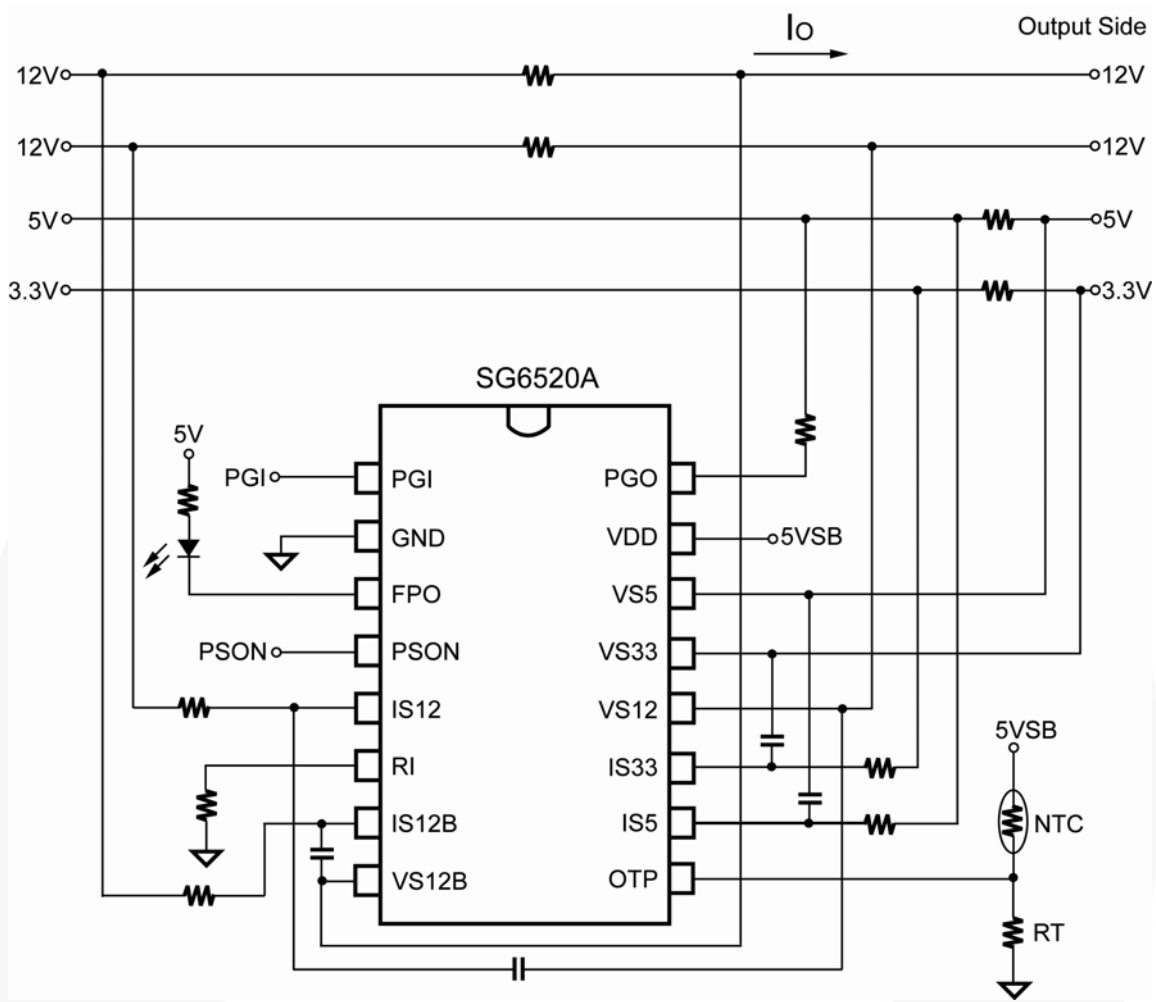
Figure 1. Typical Application
