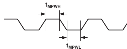
Figure 3. MCLK_I Timing
