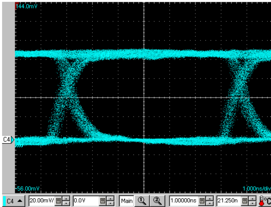
Figure 7. Eye Diagram
