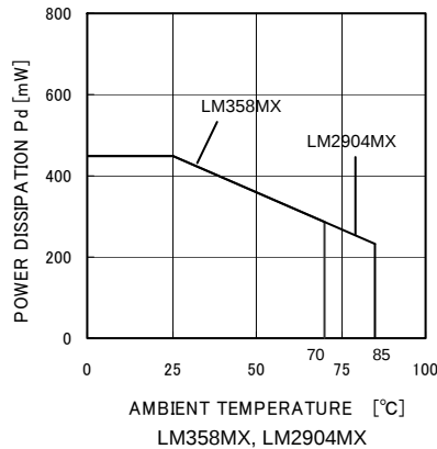
Power Dissipation
