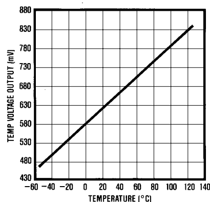
Figure 2. REF02 Temperature/Voltage Output vs. Temperature
