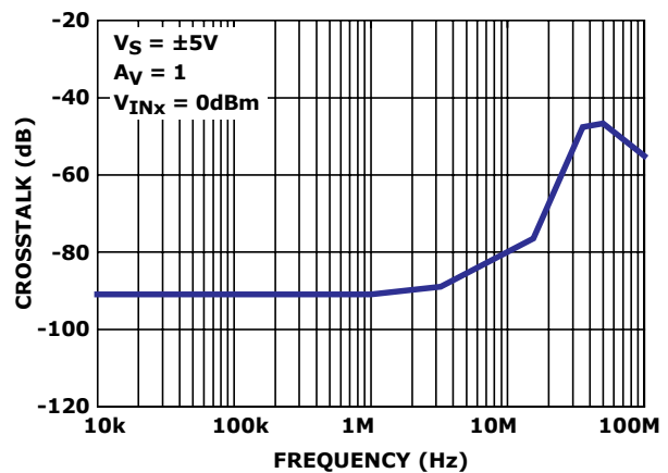
FIGURE 26. CHANNEL SEPARATION
