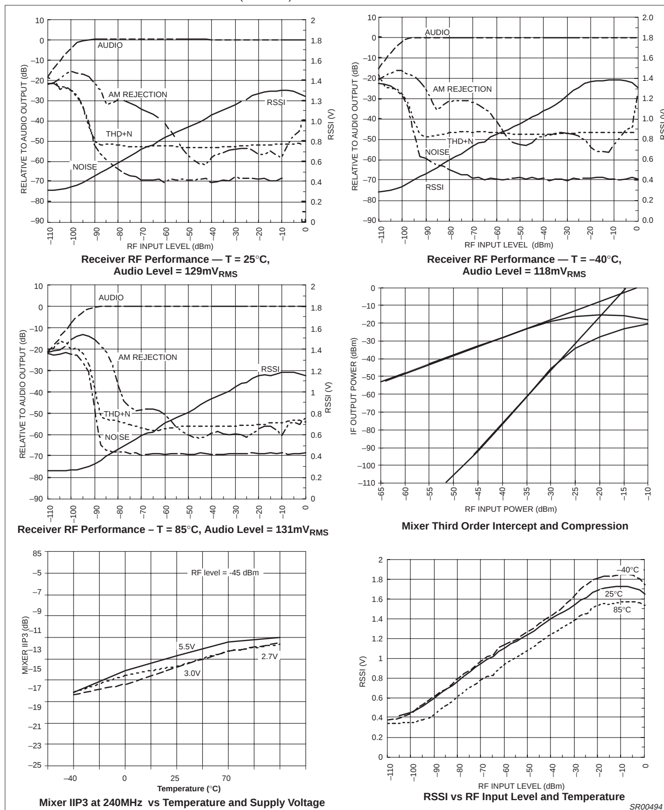
Figure 4. Performance Characteristics
