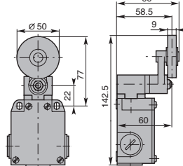
Rubber Roller Lever
