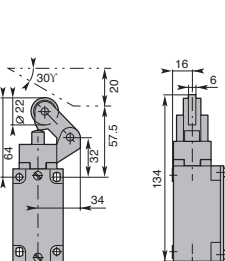
One way Roller
