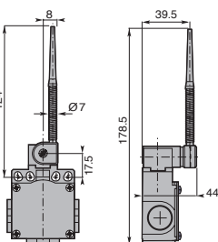
Nylon Actuator with Stainless Steel Spring
