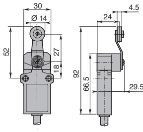
Roller Lever
