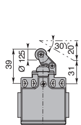
Plastic Roller
