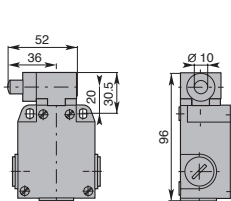
Stainless Steel Lateral Plain Plunger
