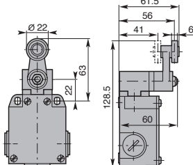
Nylon Roller Lever
