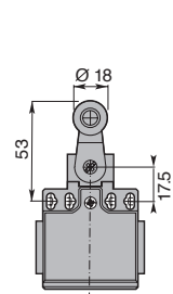
Nylon Roller Lever
