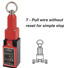
01 Slow action make before break 1NO+1NC
