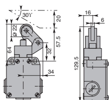
Adjustable Rubber Roller Lever
