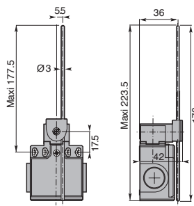
Adjustable Stainless Steel Rod Lever
