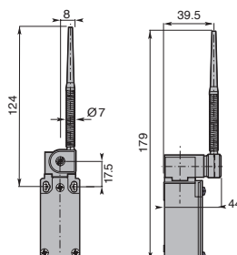
Nylon Actuator, Stainless Steel Spring
