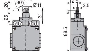
Steel Roller Plunger
