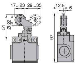
Plastic Roller on Metal Plunger
