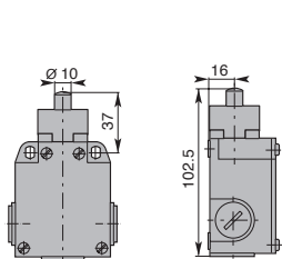
Plain Plunger
