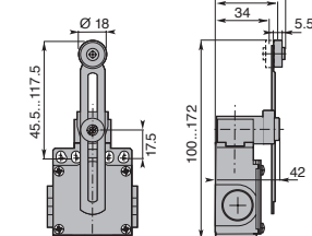
Adjustable Roller Lever
