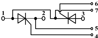
Circuit
