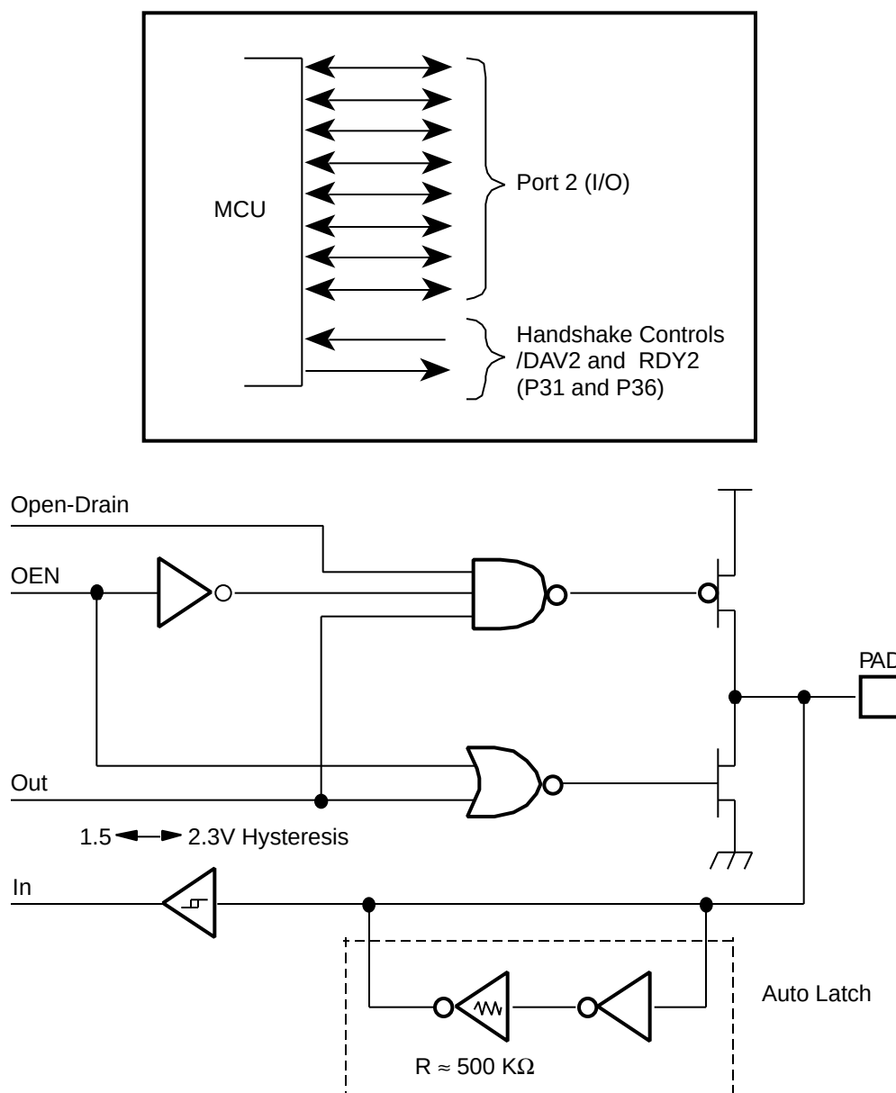
Figure 20. Port 2 Configuration
