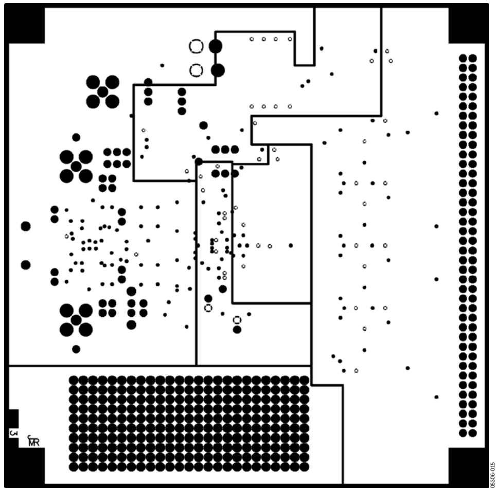
Figure 15. Layer 2 Copper
