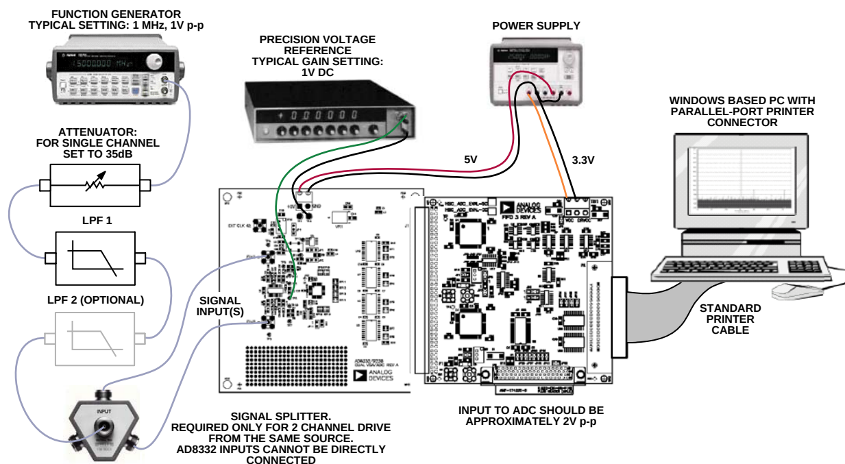
Figure 6. Test Interconnections
