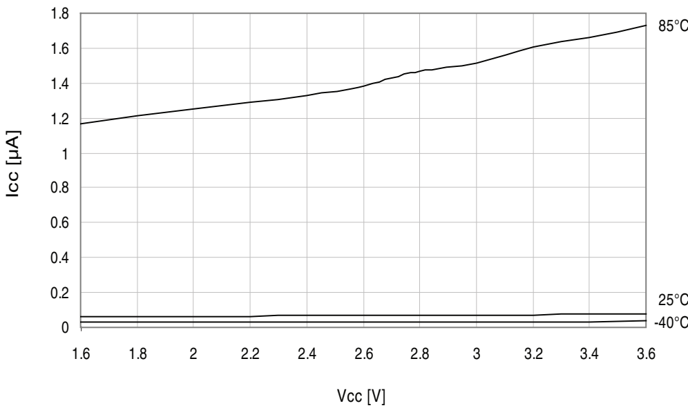
Figure 37-271. Power-down mode supply current vs. V_{CC} . All functions disabled.
