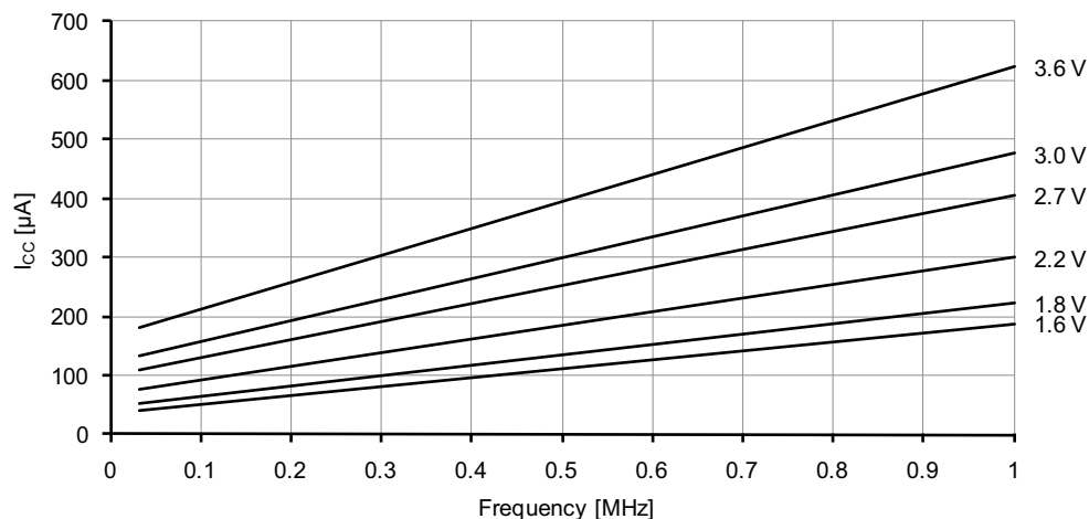
Figure 37-172. Active supply current vs. frequency.
