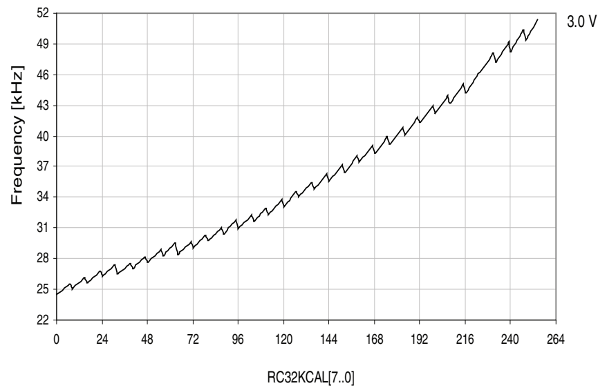
Figure 37-157. 32.768kHz internal oscillator frequency vs. calibration value.
