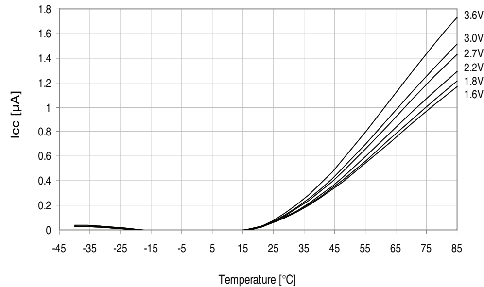
Figure 37-270. Power-down mode supply current vs. temperature. All functions disabled.
