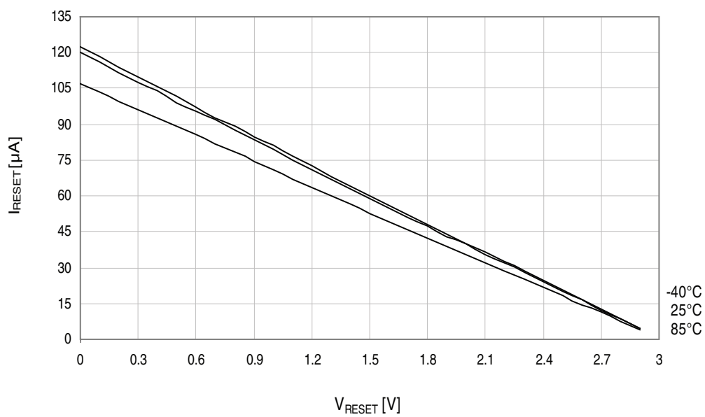
Figure 37-319. Reset pin pull-up resistor current vs. reset pin voltage.
