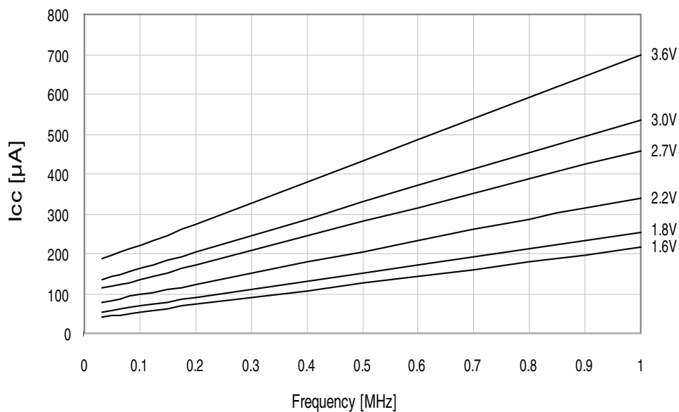
Figure 37-257. Active supply current vs. frequency.
