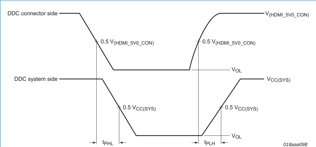
Fig 16. Propagation delay DDC, DDC connector side to DDC system side
