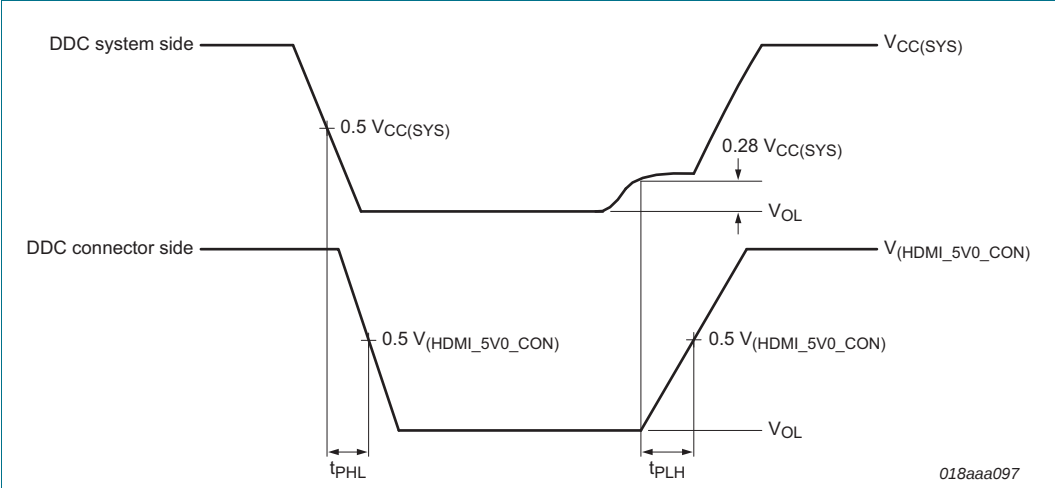
Fig 15. Propagation delay DDC, DDC system side to DDC connector side
