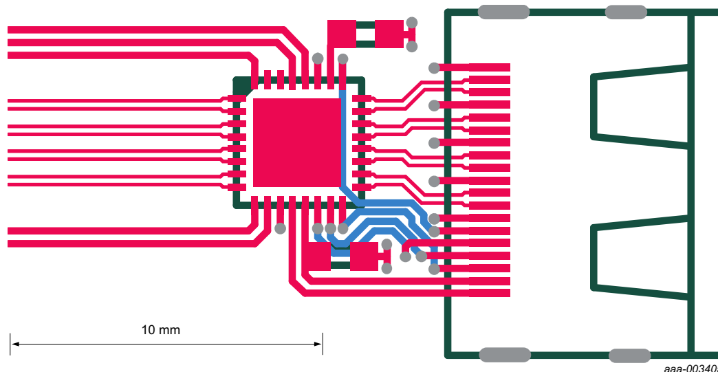
Fig 28. Application of the IP4786CZ32S showing optimized HDMI type-C connector routing
