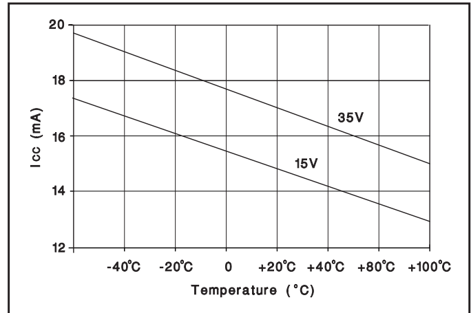
Figure 1. I_{CC} vs. temperature.
