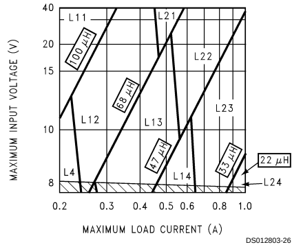
FIGURE 4. LM2675-3.3
