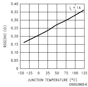
Drain-to-Source Resistance
