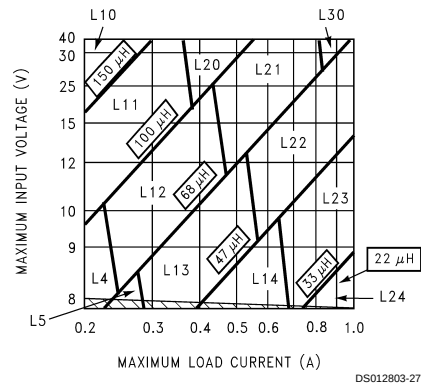
FIGURE 5. LM2675-5.0
