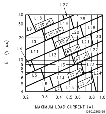
FIGURE 7. LM2675-ADJ
