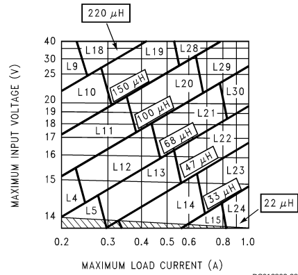
FIGURE 6. LM2675-12
