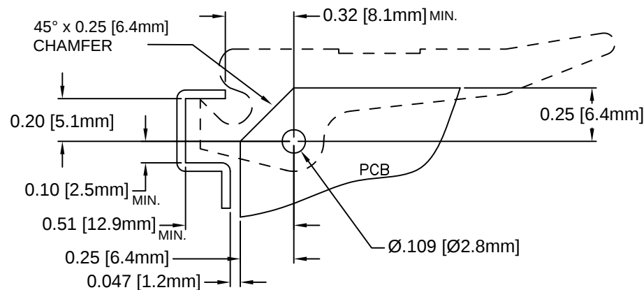
Recommended Application Layout
