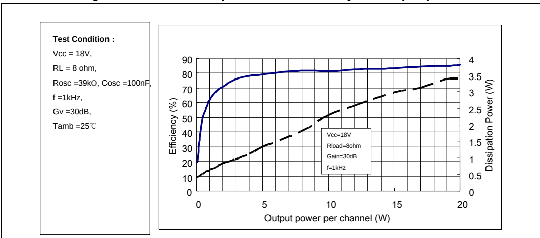
Figure 11. Power dissipation and efficiency vs. output power
