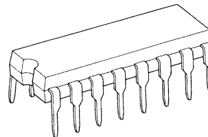
DIP16-P-300-2.54A
