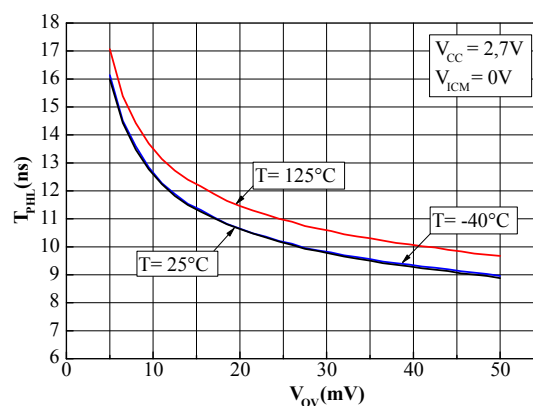
Figure 16. Propagation delay vs. overdrive with negative transition, V_{CC} = 2.7\text{V}
