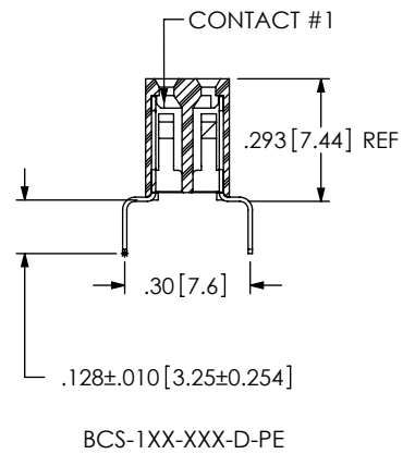
FIG 4 -PE/-PE-BE (SEE SHEET 3 FOR IN-PROCESS)
